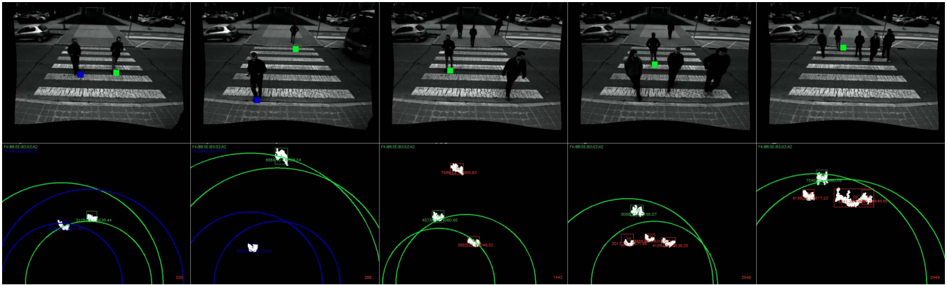
Fig. 4. Upper row: left image with color-coded identification. Lower row: XZ-map (top-view without road points), detected blobs and RSSI circumferences. Each tag is labeled with a different color.
