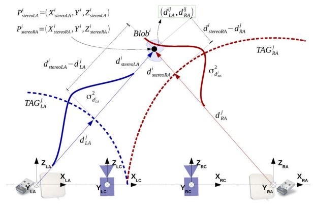
Fig. 3. Graphical representation of the new metric defined between a 3D object and the tag detected by both antennas.
